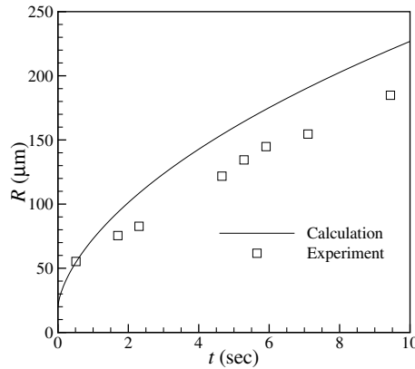
Fig. 9. Comparison of bubble growth between ALE calculation with the experimental data of Han and Yoo [41]. The experimental conditions correspond to: p_a^* = 0.04605 , Re = 1.21 \times 10^{-10} , Ca = 78.57 , \beta = 0 , k^* = 4.686 , A^* = 0.3551 and De = 495.0 . The numerical simulation matches all these except for \beta = 0.1 , and starts with a bubble radius of R_0 = 20 \mu\text{m} .
