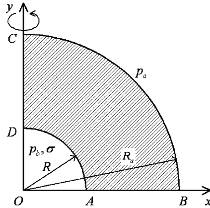
Fig. 3. Schematic of a spherical bubble of radius R surrounded by a fluid shell of outer radius R_a .
