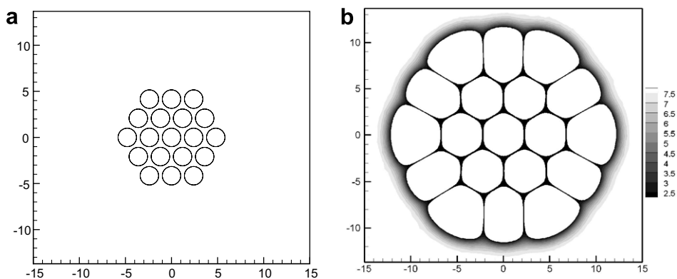
Fig. 15. Growth of a cluster of bubbles in a Newtonian melt. (a) t = 0 ; (b) t = 0.7974 . The grey-scale contours indicate the gas concentration c^* . Initially c_0^* = 8 .
