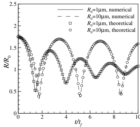
Fig. 4. Bubble oscillation in a finite extent of incompressible fluid.
