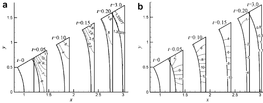
Fig. 13. (a) Distribution of the concentration of dissolved gas during foaming. The initial concentration is c_0 = 20 at t = 0 . (b) Pressure distribution within the melt. The melt is Newtonian and the process corresponds to the Newtonian curves in Fig. 12.
