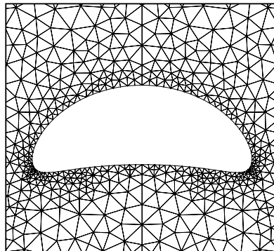
Fig. 2. Triangular mesh around a non-spherical bubble, with refined elements at the bubble tips where the surface curvature is high.
