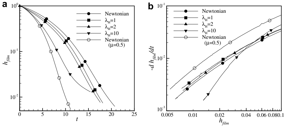
Fig. 17. Thinning of the film between the bubble and the free surface. (a) The film thickness h_{\text{film}} as a function of time. (b) The thinning rate as a function of h_{\text{film}} . Viscoelastic melts with three relaxation times are compared with a Newtonian melt of the same total viscosity \mu . A Newtonian melt with the solvent viscosity \mu_s is also shown.
