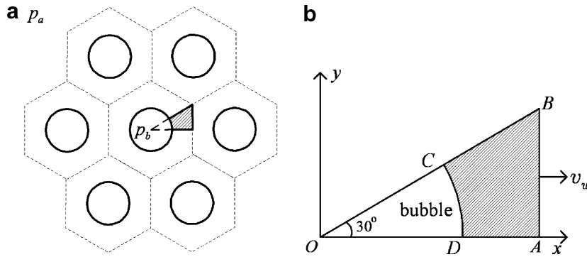
Fig. 10. (a) Hexagonal cells in a monodisperse foam. (b) The computational domain is a part of the periodic cell.
