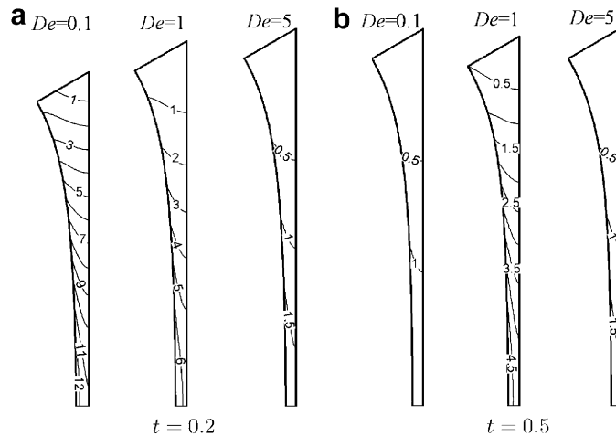
Fig. 14. Contours of the tensile stress \tau_{yy} in the viscoelastic film. (a) Buildup of \tau_{yy} toward the end of the rapid expansion stage, and (b) its subsequent relaxation in the film drainage stage.
