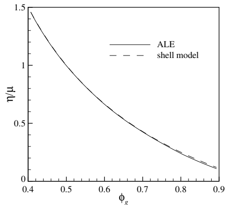
Fig. 11. Expansion viscosity of a 2D foam. The solid curve is computed from a 2D ALE simulation using Eq. (32), while the dashed one represents Eq. (33).
