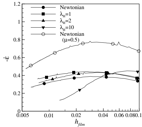
Fig. 18. Strain rate \dot{\epsilon} for the biaxial extension in the film as a function of the film thickness.
