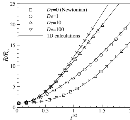
Fig. 8. Comparison of bubble growth for different De between ALE calculations (symbols) and previous 1D calculations of Feng and Bertelo [8]. The dimensionless parameters are: p_a^* = 1 , Re = 10^{-6} , Ca = 2.5 , \beta = 0.1 , k^* = 0.01 and A^* = 0.11 . The melt is of infinite expanse in the 1D calculations.
