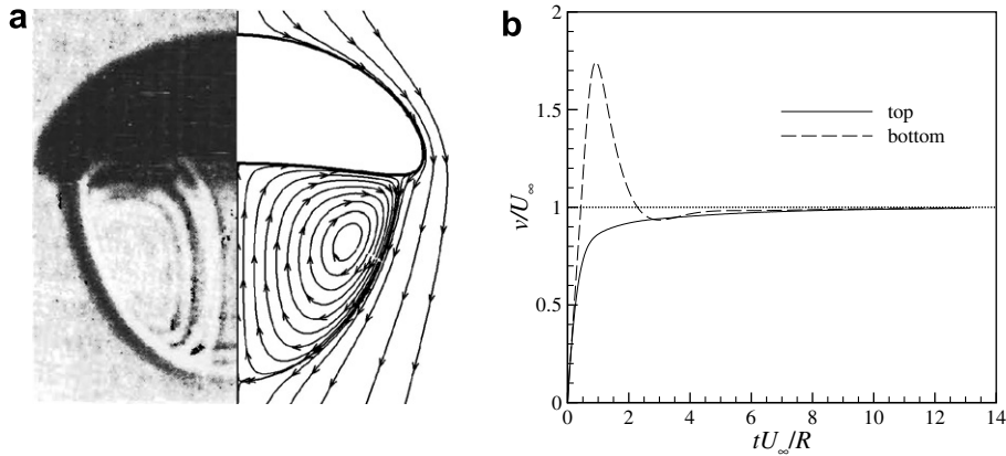
Fig. 6. (a) The steady-state bubble shape. The left half is from the experiment of Hnat and Buckmaster [38], while the right half is our simulation. The streamlines are in close agreement as well. (b) The instantaneous velocity at the top and bottom of the bubble, scaled by the experimental terminal velocity U_\infty .
