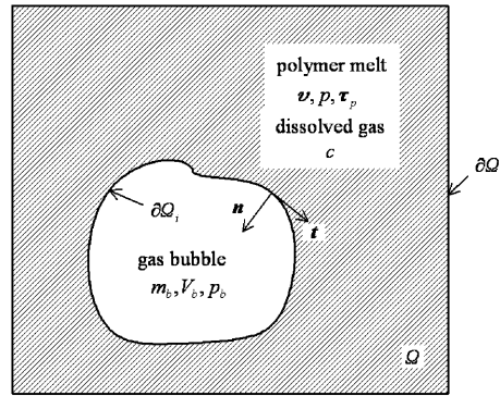
Fig. 1. Schematic of a gas bubble in a polymer melt. \Omega is the computational domain with inner boundary \partial\Omega_i and outer boundary \partial\Omega_o . Pressure p , velocity \mathbf{v} , polymer stress \boldsymbol{\tau}_p and gas concentration c are to be solved in the polymer melt, while the bubble mass m_b , volume V_b and pressure p_b need to be calculated for the bubble.
