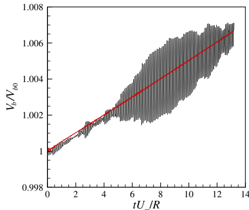
Fig. 7. The bubble volume V_b , scaled by the initial volume V_{b0} = \frac{4}{3}\pi R^3 , increases during the rise. The thick line is for a finer mesh with 100 elements on the bubble surface, while the oscillatory trajectory is for a coarser mesh with 50 surface elements.
