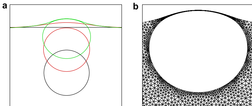
Fig. 16. A bubble pressing against a free surface in a Newtonian melt. (a) Snapshots of the interfacial morphology at t = 0, 9.85 , and 20.45 . (b) Computational mesh around the bubble at t = 20.45 .
