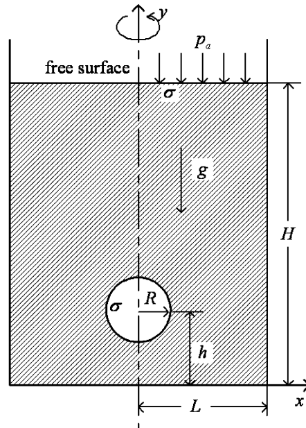
Fig. 5. Schematic of the computational domain for the rising bubble.
