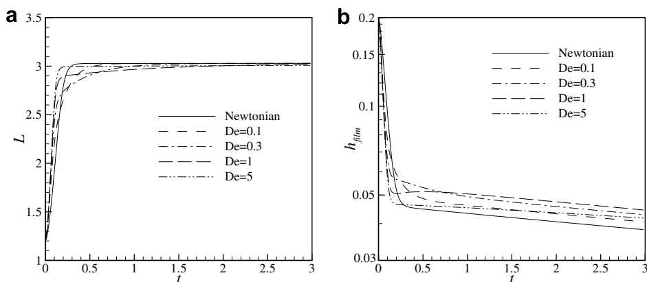
Fig. 12. (a) Temporal growth of the foam size indicated by L = \overline{OA} . (b) Evolution of the film thickness h_{\text{film}} = \overline{DA} . For all non-Newtonian melts \beta = 0.5 .
